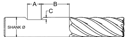
Single Weldon
